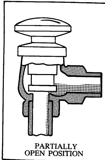
RADIATOR VALVE
