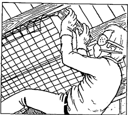
CHICKEN WIRE SUPPORT USED
