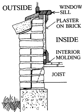
EXISTING 10" WALL, CROSS SECTION OF TYPICAL MASONRY WALL
