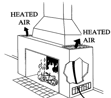
CONVECTION DEVICE FOR INCREASING FIREPLACE EFFICIENCY
